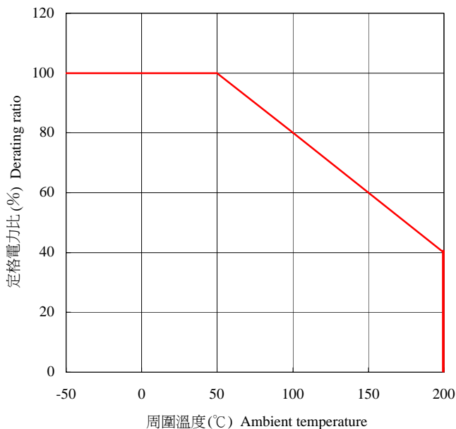
負載減輕曲線圖 Power Derating Curve
