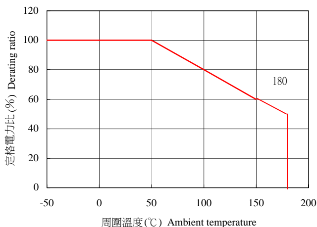
負載減輕曲線表 Power Derating Curve
