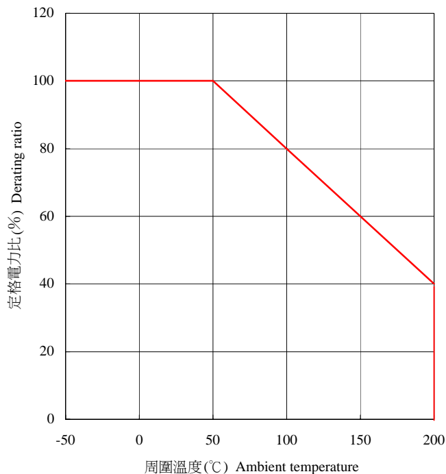
負載減輕曲線圖 Power Derating Curve
