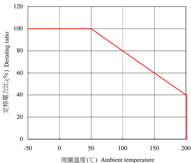
負載減輕曲線圖 Power Derating Curve
