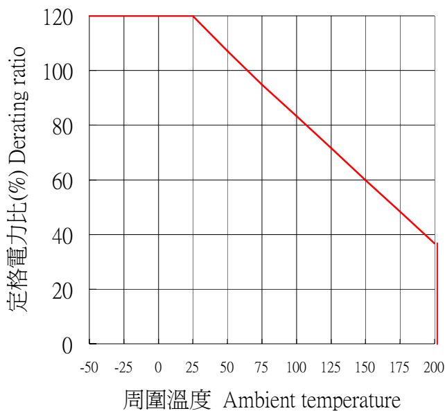
負載減輕曲線表 Power Derating Curve
